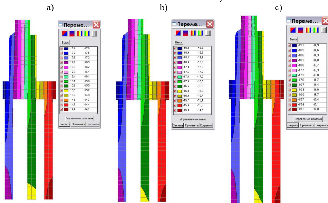
Fig. 4. Isolines and isofields of vertical displacements in a fragment of the abutment model: a) 1st combination; b) 2nd combination; c) 3rd combination
