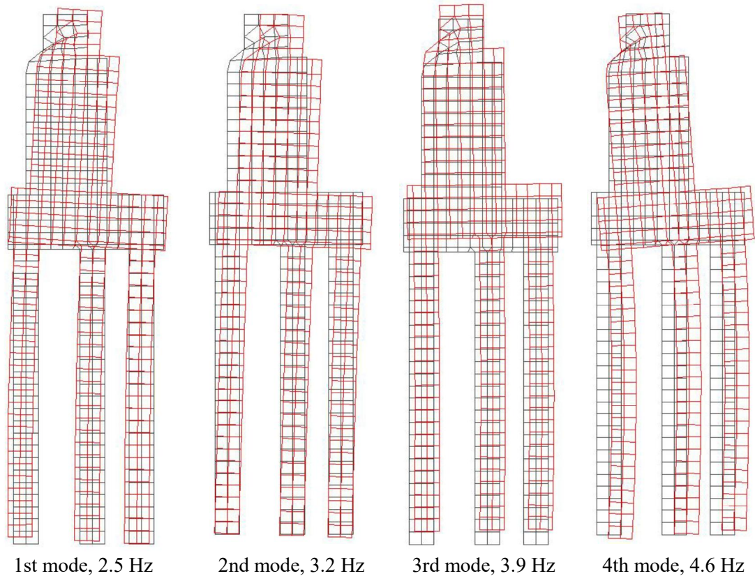
Fig. 5. Modes and frequencies of natural vibrations of an abutment
