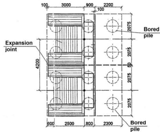
Fig 1. View of the abutment from above
