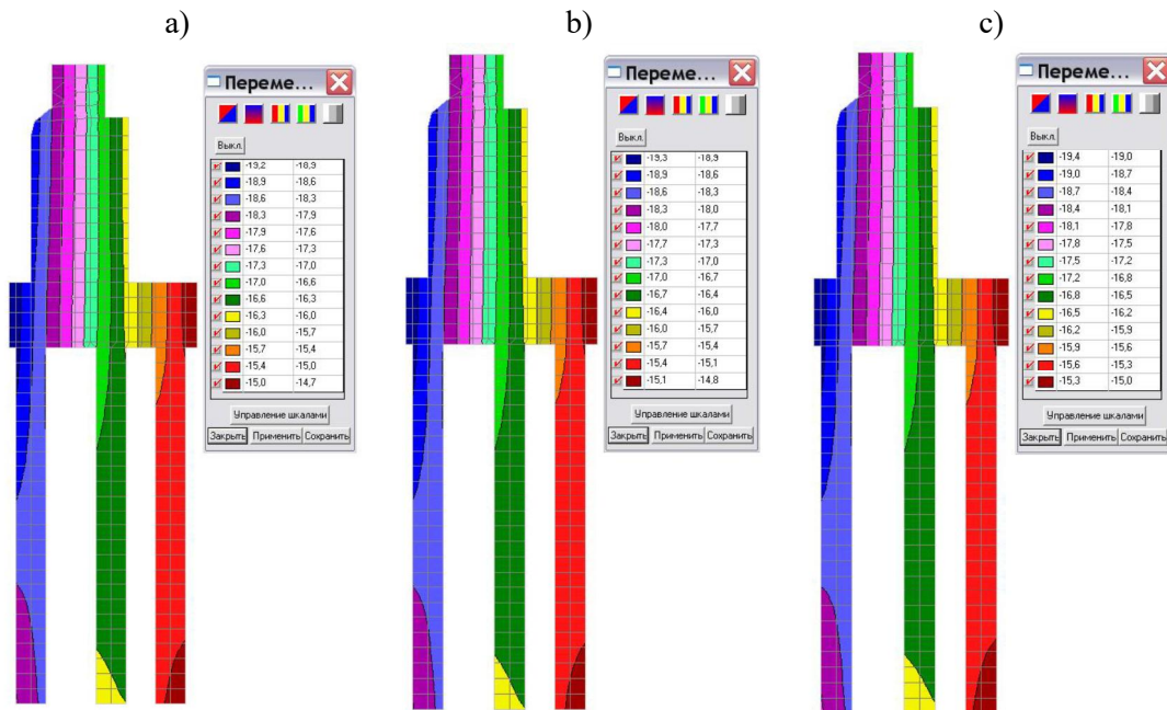
Fig. 6. Isolines and isofields of vertical dynamic displacements in a fragment of the abutment model: a) 1st combination; b) 2nd combination; c) 3rd combination
