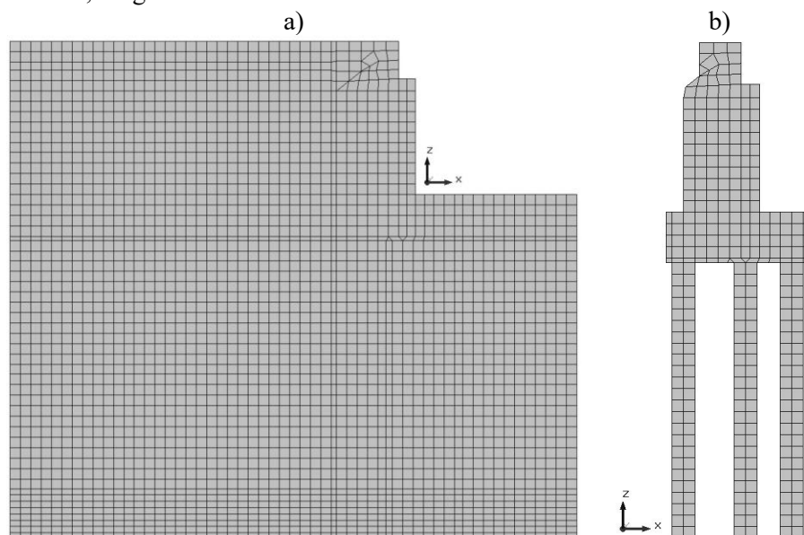
Fig. 3. General view of the model (a) and a fragment of the model (abutment) (b)
