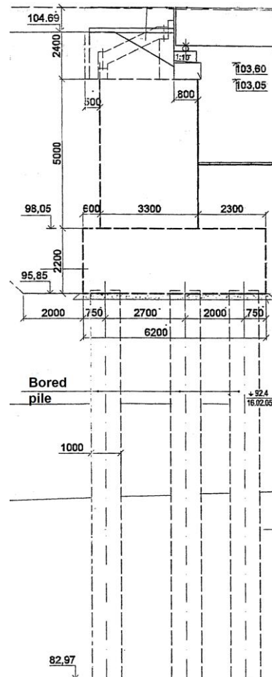
Fig. 2. General view of the abutment
